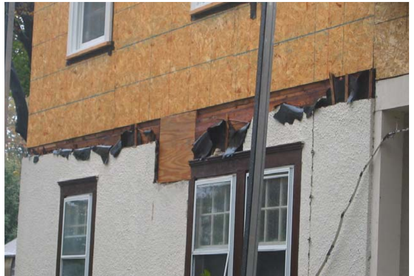
October 28, 2008 – Water seepage through exposed seams between first and second floors (42 Maple Ave.) Top – living room; above – North elevation; below – South elevation.
